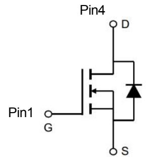
Pin2,3,5,6,7 N-Channel MOSFET
